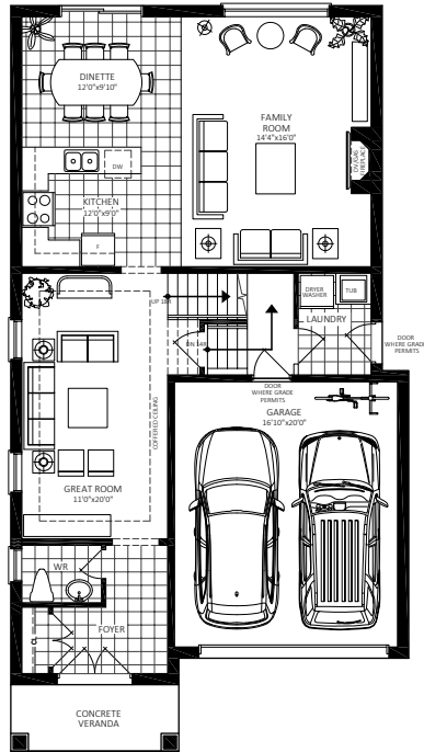
First Floor Elev. A
